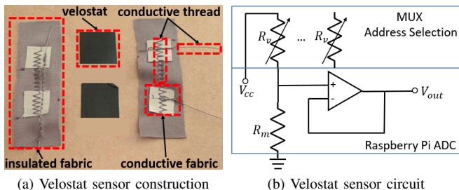
Fig. 3: Velostat force sensor construction and circuit layout
