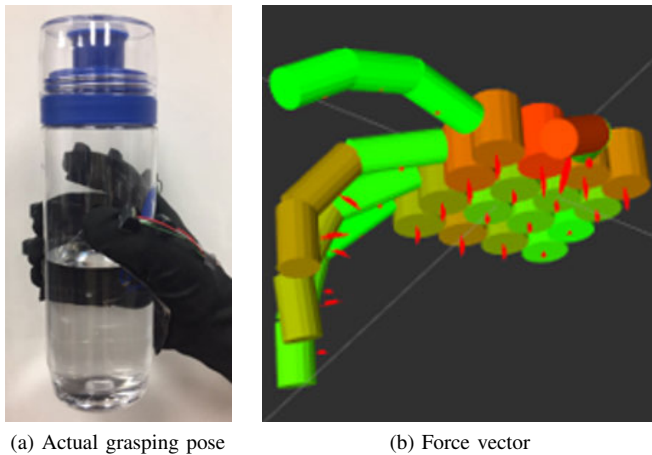
Fig. 10: Grasp of half-full bottle and captured pose and force vector
