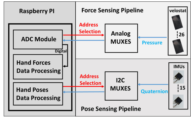
Fig. 2: Overall system schematic
